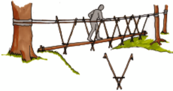
Friction bridge
