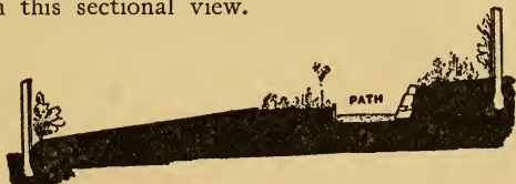
Fig. 36.—Dealing with a transverse slope
